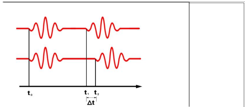
Illustration 2: Transit-time measuring principle
