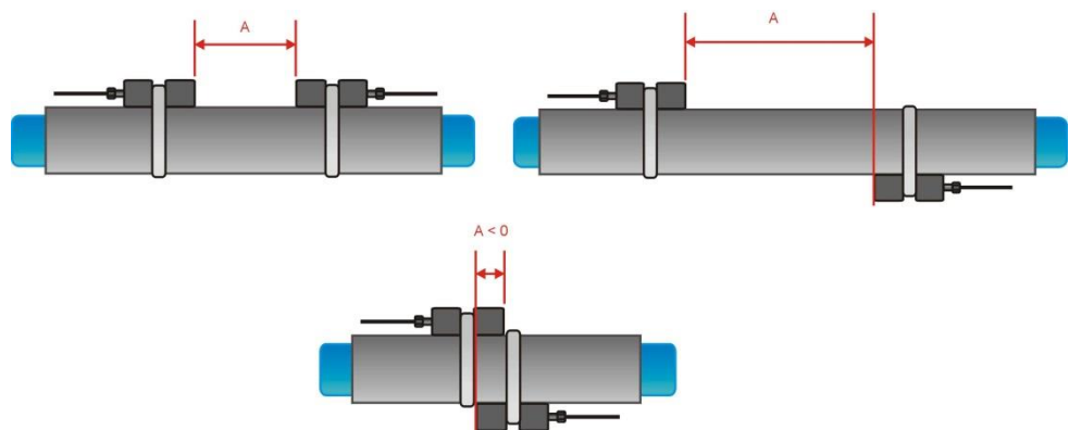
Illustration 6: Correct positioning of the sensors
